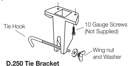
D.250 Tie Bracket
